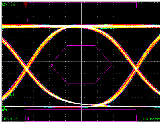
Signal pattern: PRBS 7
