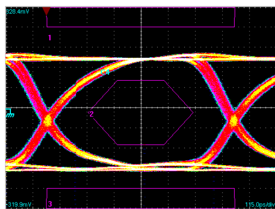
Signal pattern: PRBS 7 Input Power: -19 dBm
